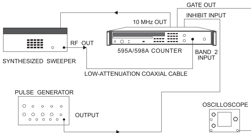
Figure 6-13. Band 2 Averaging Error Test Setup
