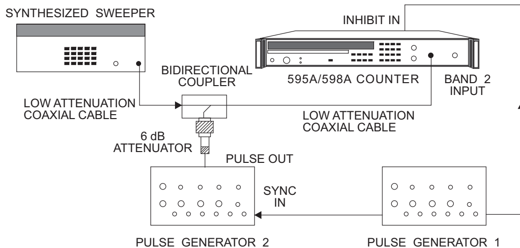
Figure 6-17. Band 2 Maximum Video Test Setup
