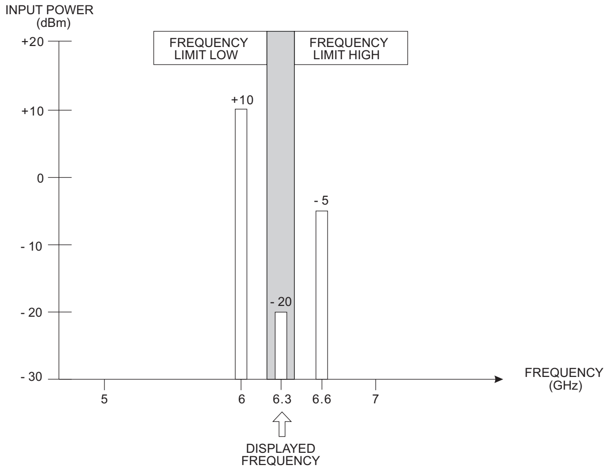
Figure 3-13. Frequency Limits
