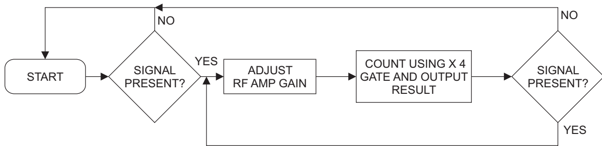
Figure 3-9. Band 1 RF Converter Lock Process Flow
