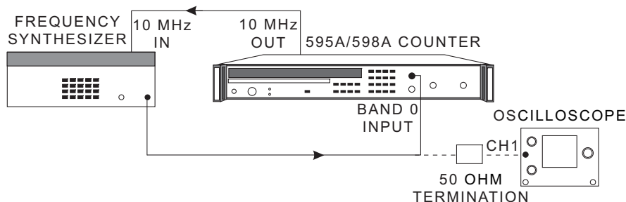
Figure 6-2. Band 0 Range and Sensitivity Test Setup 1 (100 Hz to 10 MHz)
