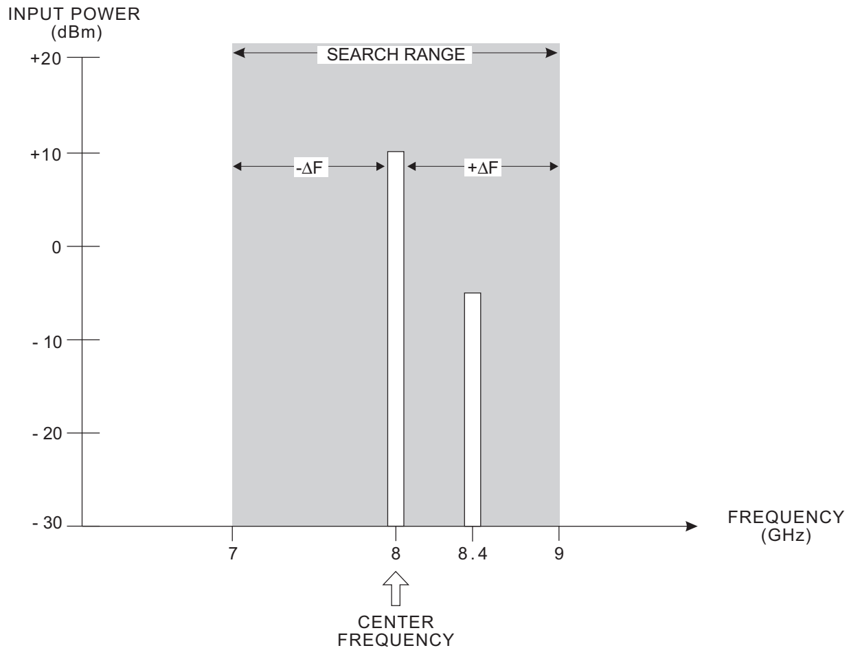
Figure 3-14. Center Frequency
