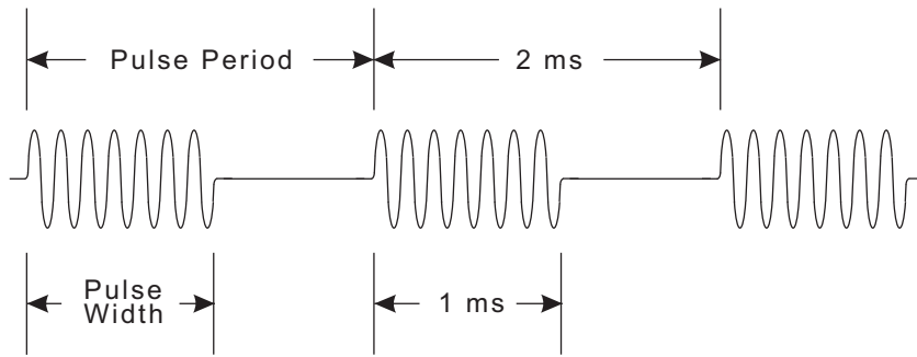
Figure 3-12. Pulsed Signal
